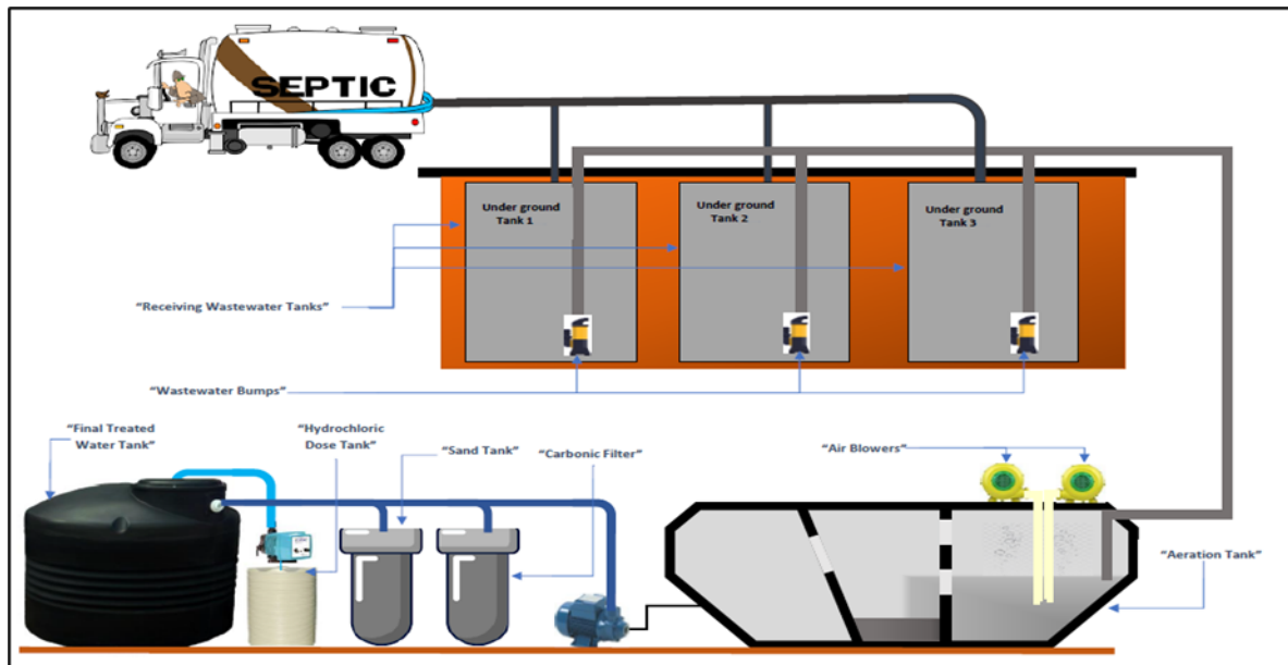
Wastewater Treatment Plant (Activated Sludge Technology)
